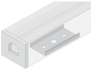
U-Clip Total Dimensions: 0.64 × 0.64 (H x W)
